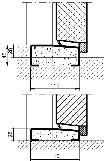
half sill
